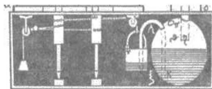
1b-rasm. Fizikaviy jarayonning amalga oshishi.
